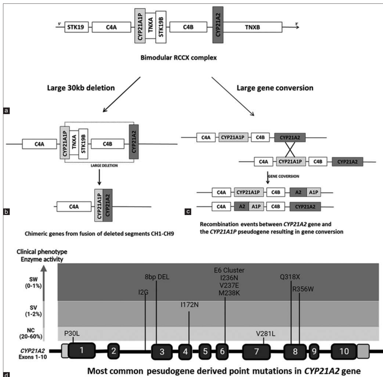
Figure 1: Schematic representation of molecular mechanisms in 21-OH deficiency. a) Bimodular RCCX complex with CYP21A2 , C4B , TNXB and STK19B genes. b) Large 30 kb deletion encompassing 5' of CYP21A1P and 3' of CYP21A2 genes. The remaining segment of these two genes fuse together to form different chimeric genes. c) Large gene conversion replacing functional gene sequence partly or completely with that of pseudogene. d) The most common pseudogene derived hotspot mutations in CYP21A2 gene
